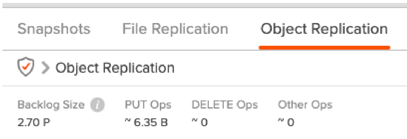
Figure 6.2 Object ReplicationHeader
