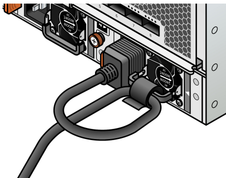
Figure 7.2 Securing the Power Cord
