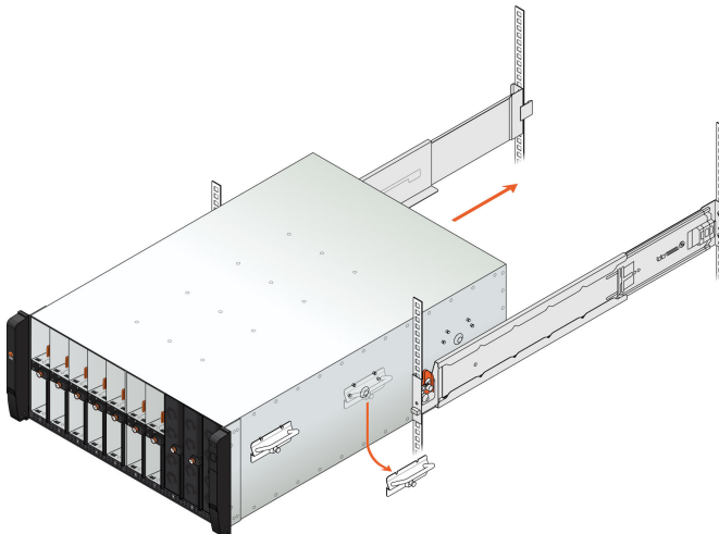
Figure 4.6 Mounting on Rack, Part 2
