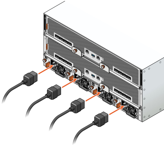
Figure 7.1 Connecting Power Cords
