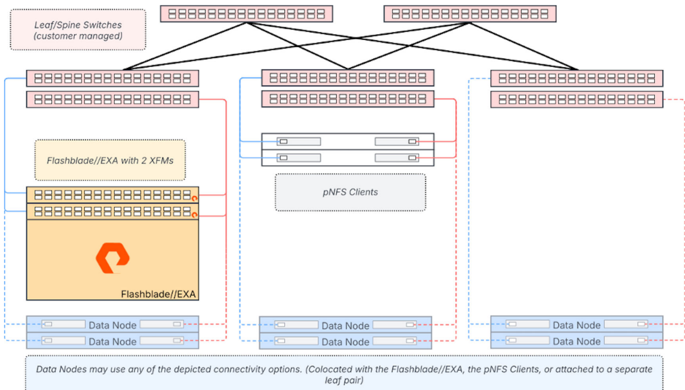
Figure 4.1 FlashBlade//EXA Connectivity
