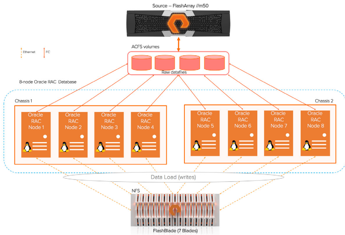
FIGURE 7. System connectivity
