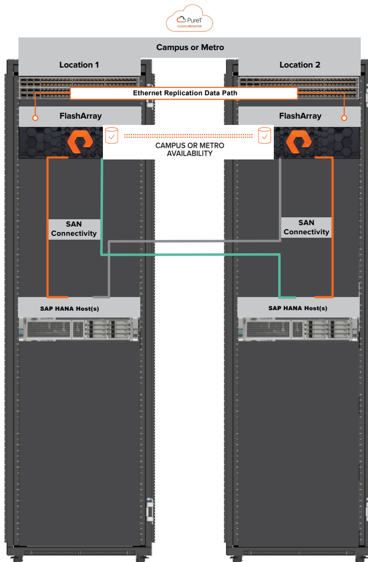
Fig. 5 ActiveCluster across campus or metro availability zones with secondary compute at the redundant site.
