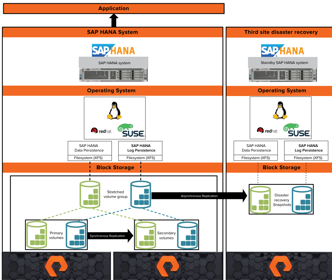
Fig. 17 Extending uniform host access to a third site for DR purposes.
