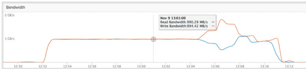
FIGURE 8. FlashBlade bandwidth during restore
