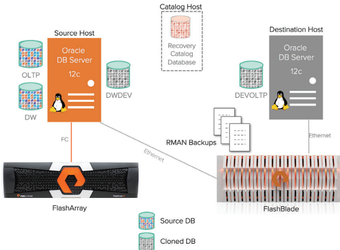
FIGURE 3. RMAN environment
