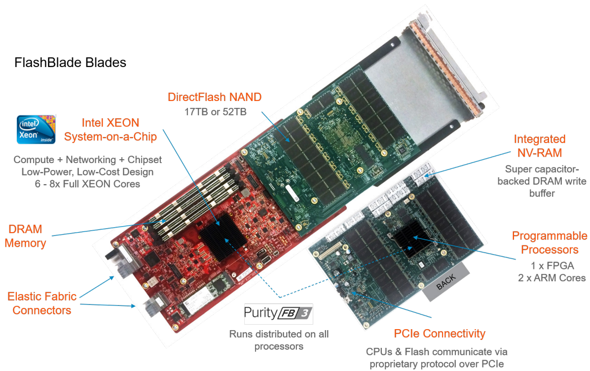
Figure 3: Anatomy of a FlashBlade.
