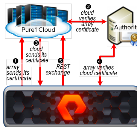
Figure 4: Mutual Authentication
