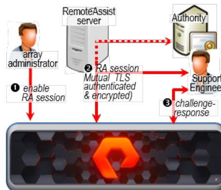
Figure 5: RemoteAssist Authentication
