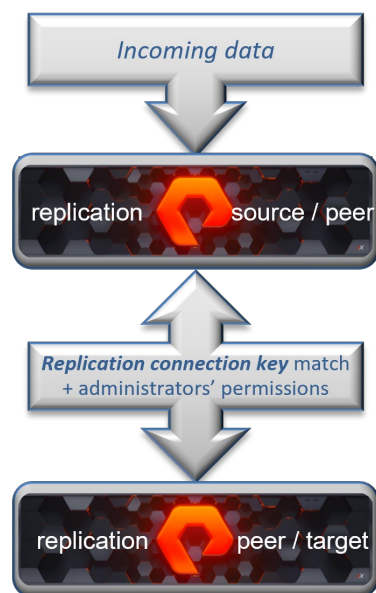
Figure 2: Replication Security
